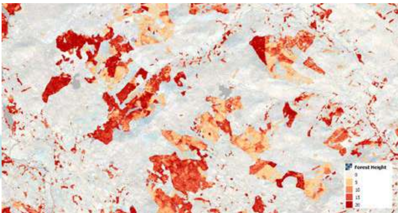
Forest height map over a site in Scotland retrieved from Sentinel-1 and -2 observations delivered by Copernicus.
