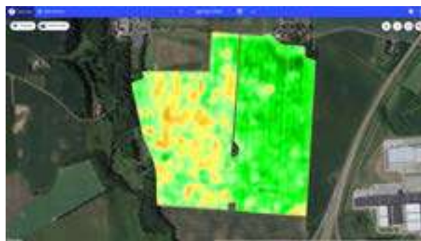
Biomass map of two fields as shown in FieldSense. Eastern Jutland, Denmark.
