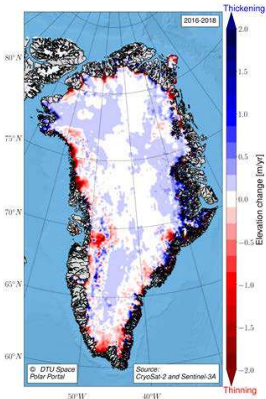
The surface elevation changes from January 2016 to December 2018, as derived operational from combining data from Cryosat-2 and Sentinel-3A.
