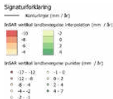
Figure 1. Vertical movement calculated from calibrated Sentinel-1 LOS data for ascending track LOS-146A (top) and LOS-66D (middle). The vertical movement is shown as a 2D product (bottom).
